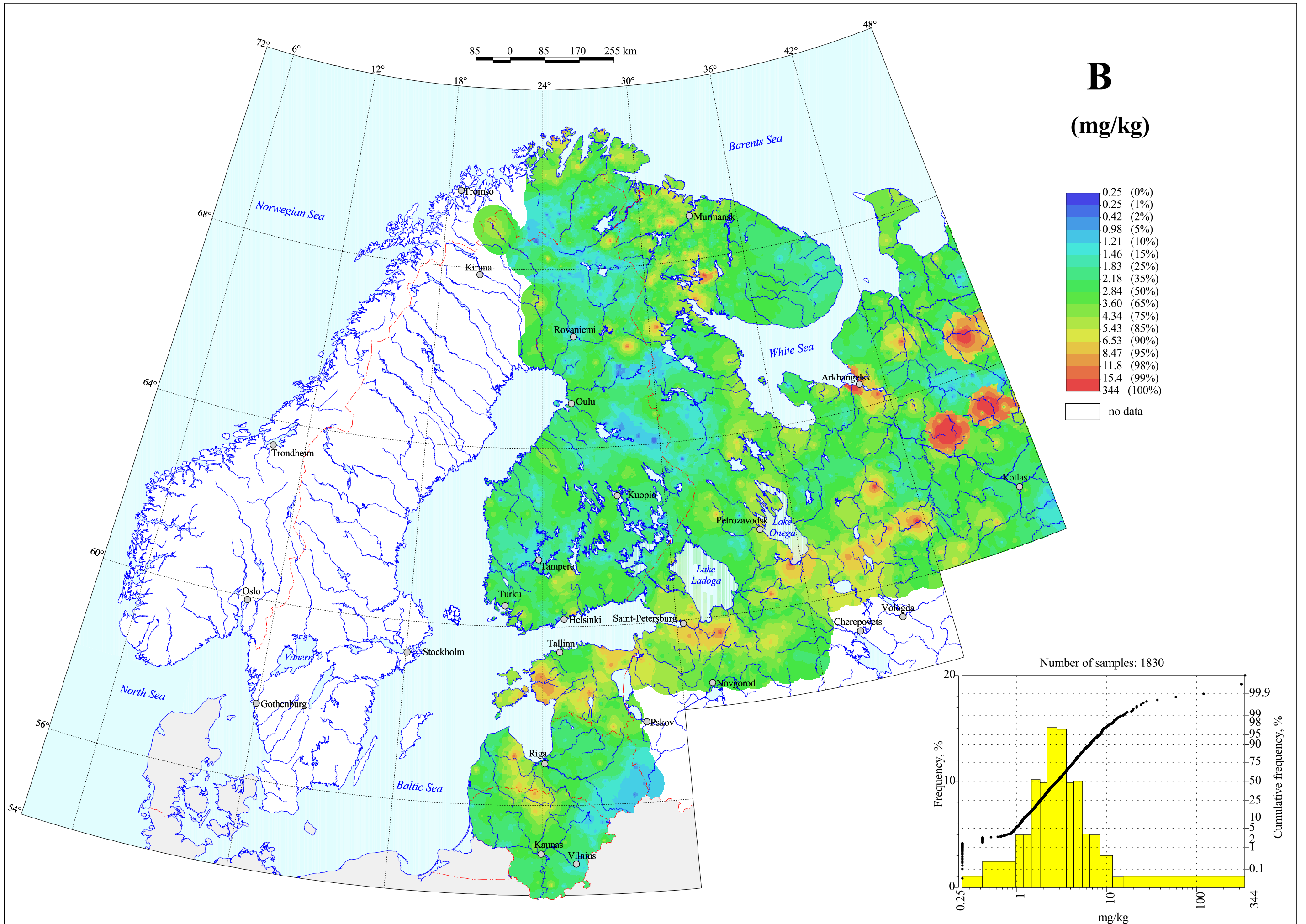
Boron in Terrestrial Moss, Total Content
